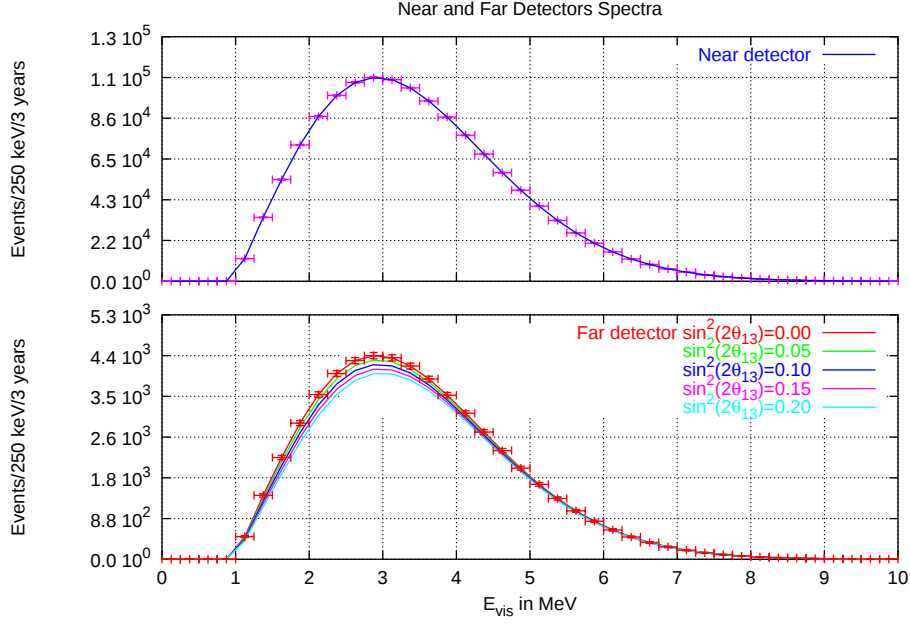
Figure 3.6: Positron spectrum (visible energy, MeV) simulated for the CHOOZ-near and far detectors
